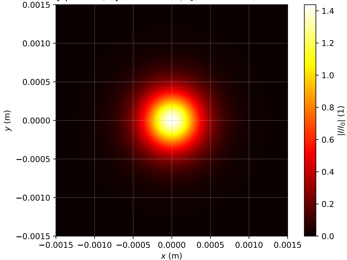
Intensity profile I(x, y, z = 3.821m)/I_0 , Pin=0.9Pcr, artificial time
